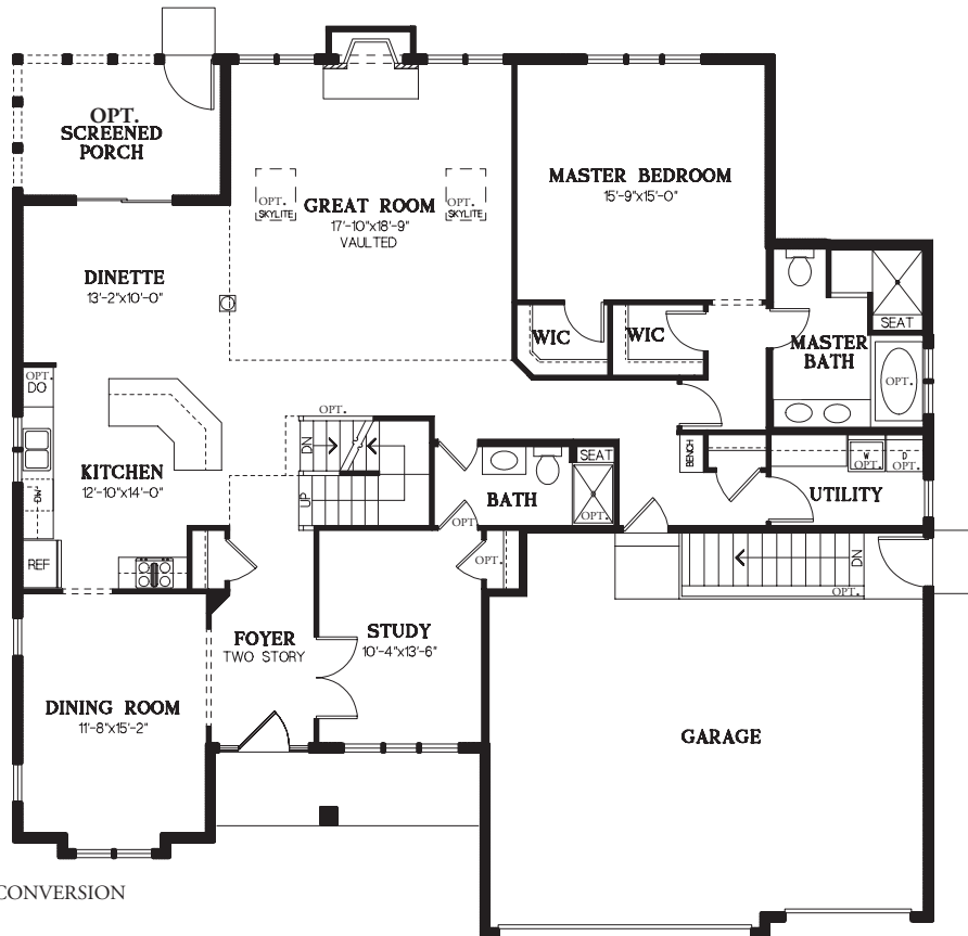
FIRST FLOOR PLAN 2013 SQUARE FEET 2758 TOTAL SQUARE FEET
